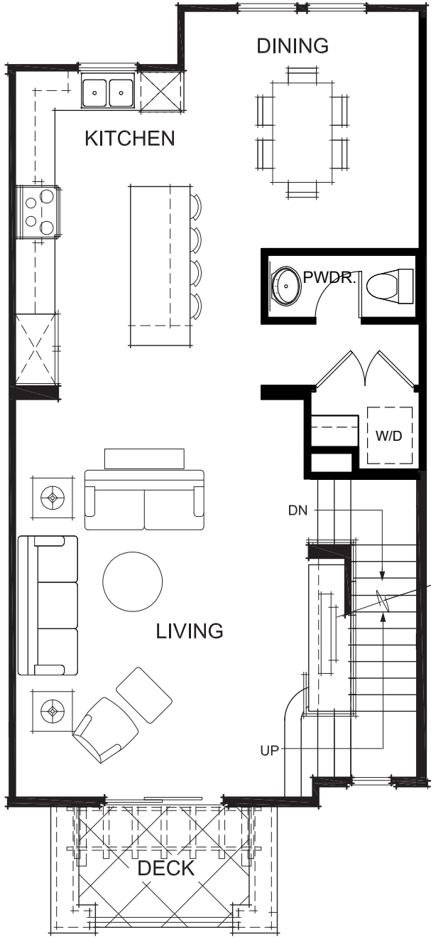
2ND FLOOR
