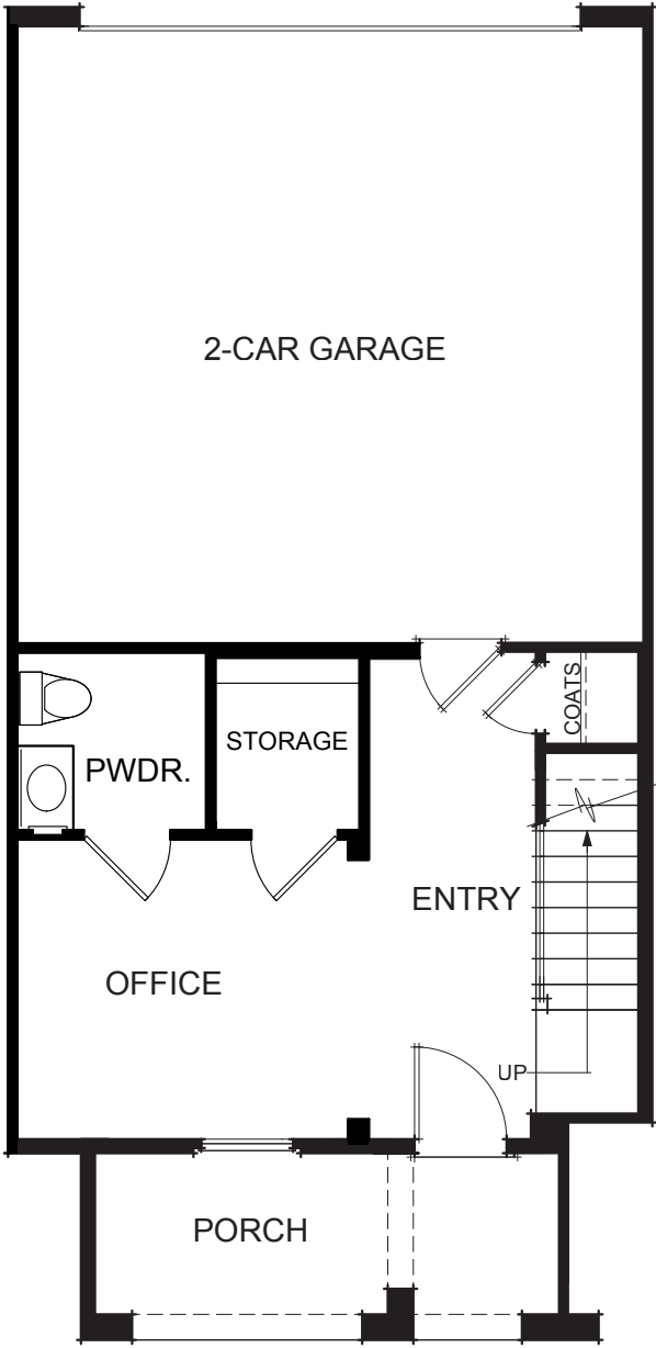
1ST FLOOR
