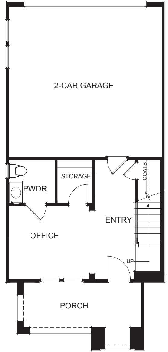
1ST FLOOR
