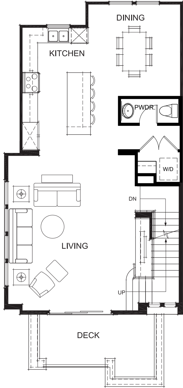
2ND FLOOR
